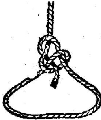
BOWLINE FOR SECURITY.
