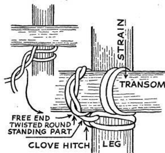
SQUARE LASHING
