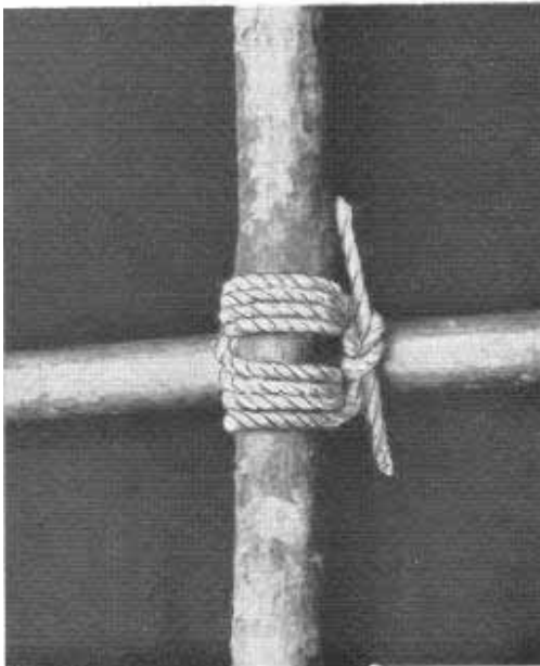
6. Lashing Complete.
