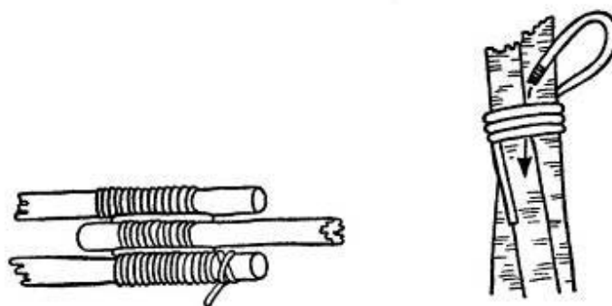
FIGURE OF EIGHT LASHING
