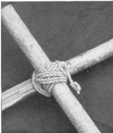
6. Finished Lashing.
