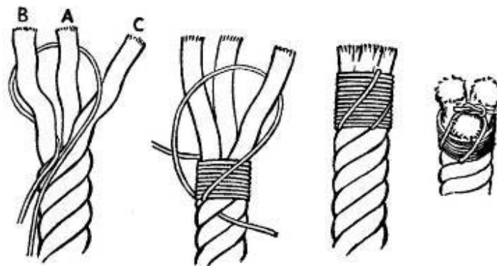
SAILMAKER'S WHIPPING
