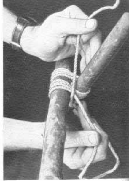
5. Start of final reef knot.
