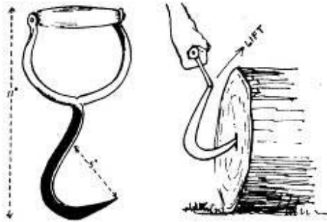
THE PULP HOOK
