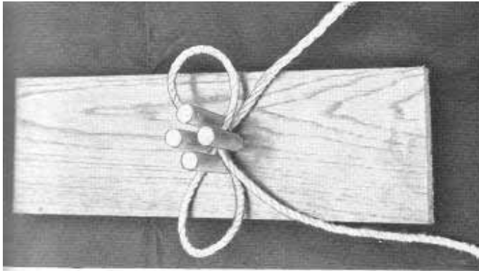
1. Four Pole Sailmaker's Lashing. Demonstration Board to Show Starting Process.
