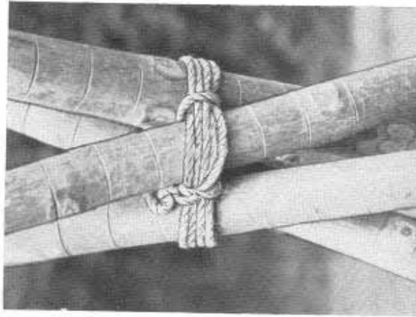
2. Four Pole Sailmaker's Lashing Complete.
