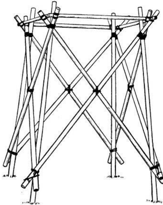
TEN MINUTE TOWER
