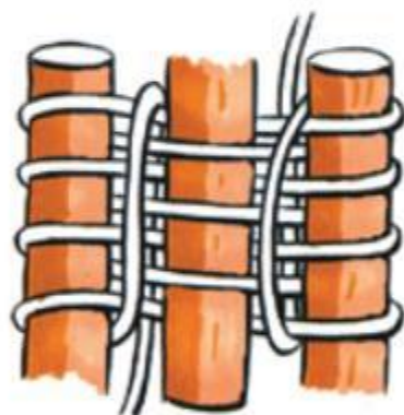
Danish Tripod lashing
