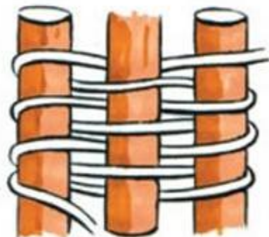
Danish Tripod lashing
