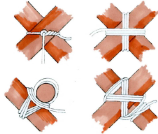
Diagonal Lashing
