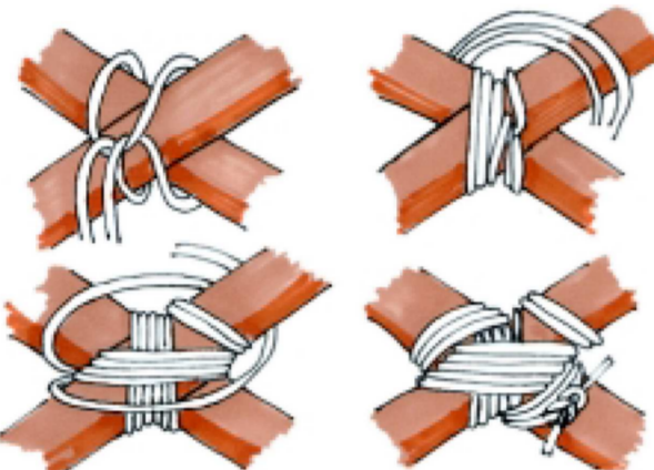
Japanese Lashing
