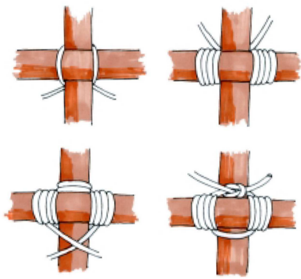
Norwegian Lashing
