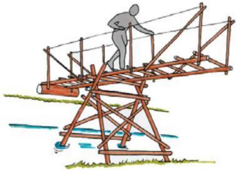
See-saw Bridge
