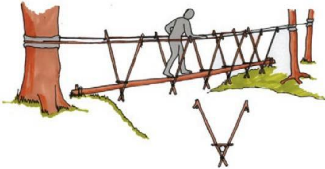
Outback Bridge
