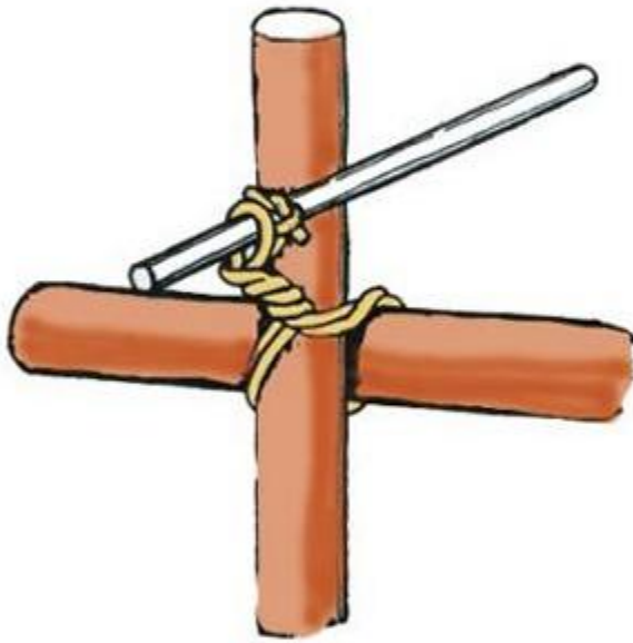
Tourniquet lashing (tightening the lashing)
