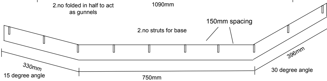
750mm
